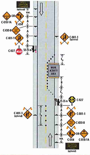
Figure 7.A: Lane Closure with TCPs - Single Lane Alternating - Short and Long Dur
